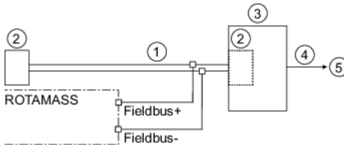
Fig. 49: Raccordement PROFIBUS PA
