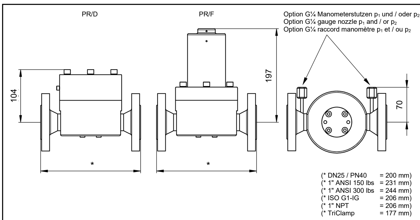
PR25: DN25 / PN40, 1" / 150 lbs / 300 lbs
