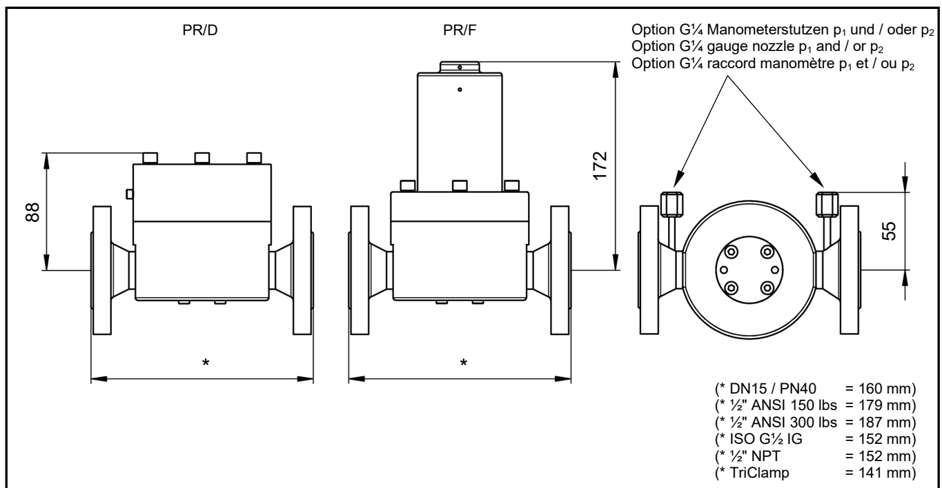
PR15: DN15 / PN40, ½" / 150 lbs / 300 lbs
